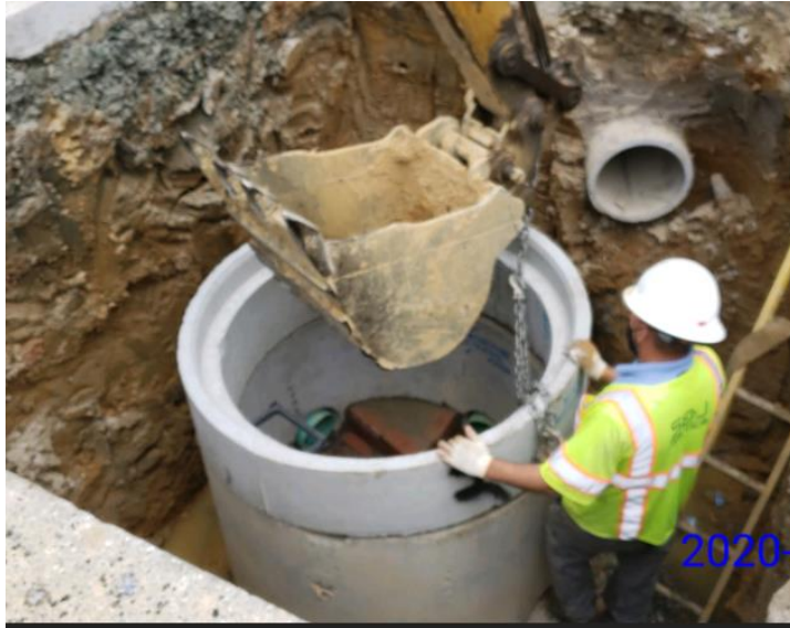
New bench for the base of Manhole S17AA_037MH being built.
