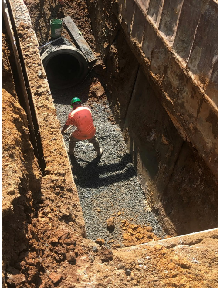
Preparing Stone Bedding for RCP Sewer Pipe
