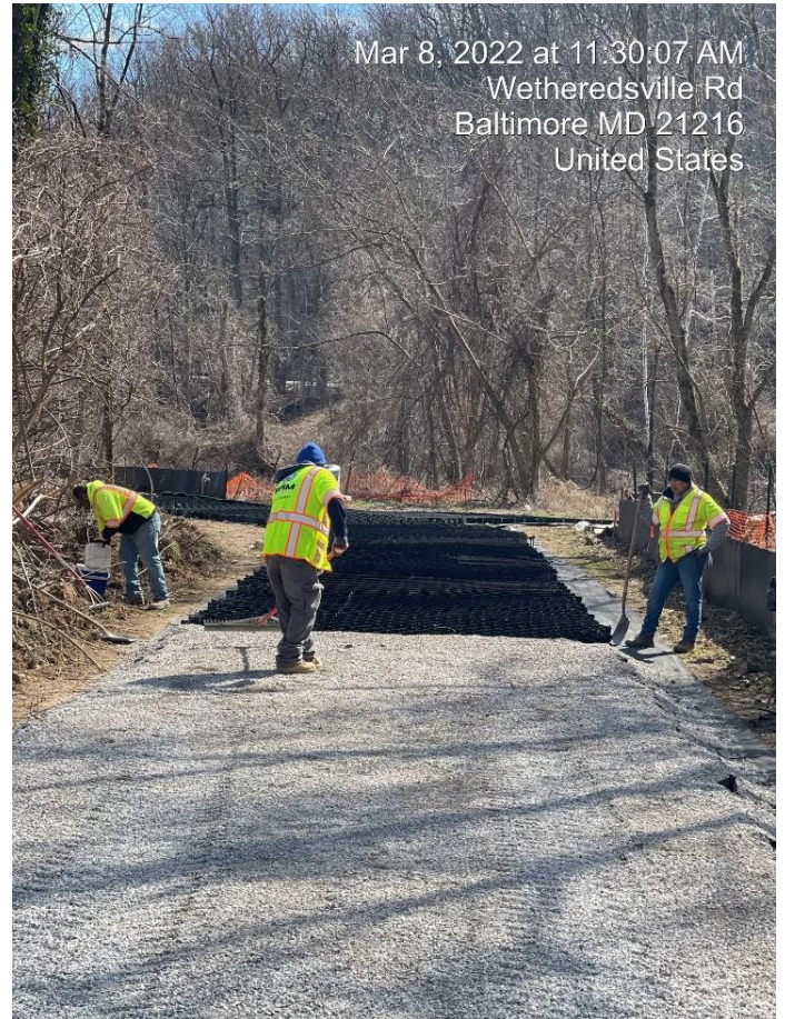
Geogrid being filled in with Stone
