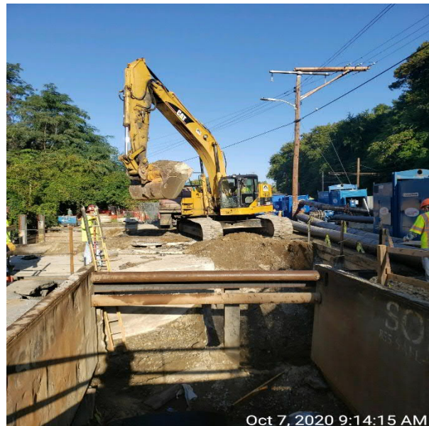
Backfill Siphon Structure B
