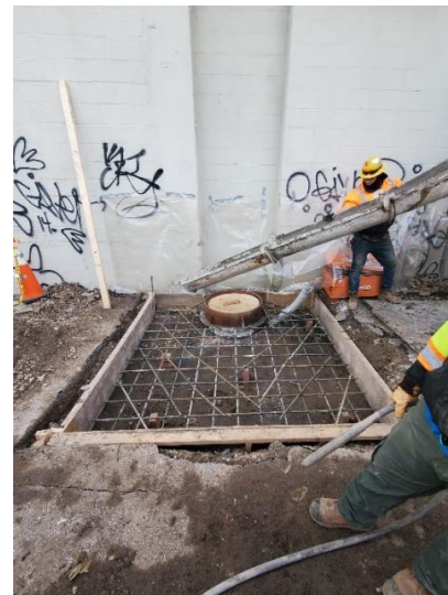
Manhole Rehab (Preston St)
