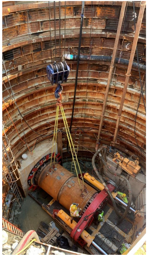
Relief sewer microtunneling underway at the intersection of Wabash Ave & W Cold Spring Ln
