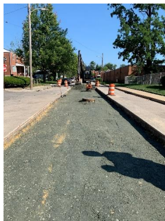
Concrete roadway restoration 3900-4000 Block of Callaway Avenue
