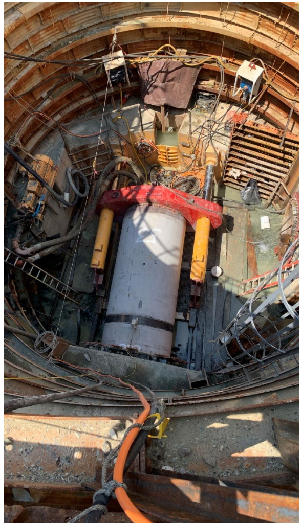
Microtunneling underway at the intersection of Wabash Ave & W Cold Spring Ln
