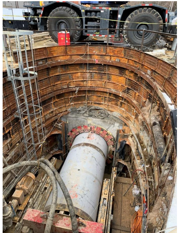
Microtunneling underway at Wabash Ave & Dorithan Road
