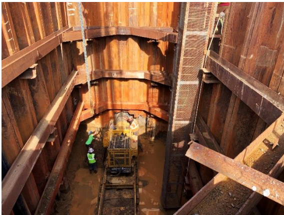
42" casing pipe being tunneled under Northern Parkway for future sewer installation
